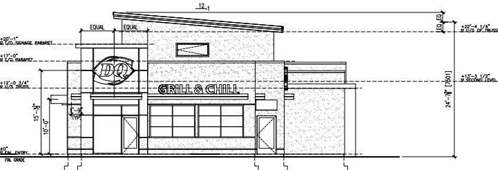
3 EAST ELEVATION 1/8"=1'-0"
