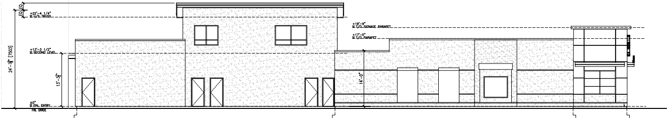
2 SOUTH ELEVATION 1/8"=1'-0"
