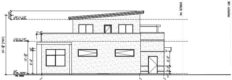
4 WEST ELEVATION 1/8"=1'-0"
