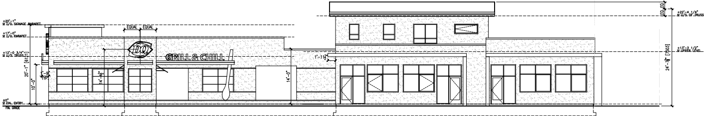
1 NORTH ELEVATION 1/8"=1'-0"
